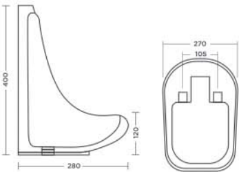
NERO Urinal L270 x W280 x H400mm MRP ₹ : 1470/-
